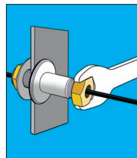
11 Push cable trough assembled gland and tighten nut.
