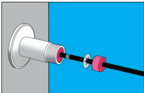
5 Push first piece of seal into place.
